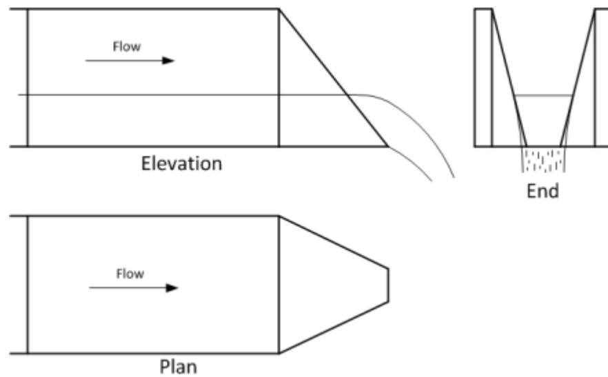
Figure 16 – H-Flume configuration
