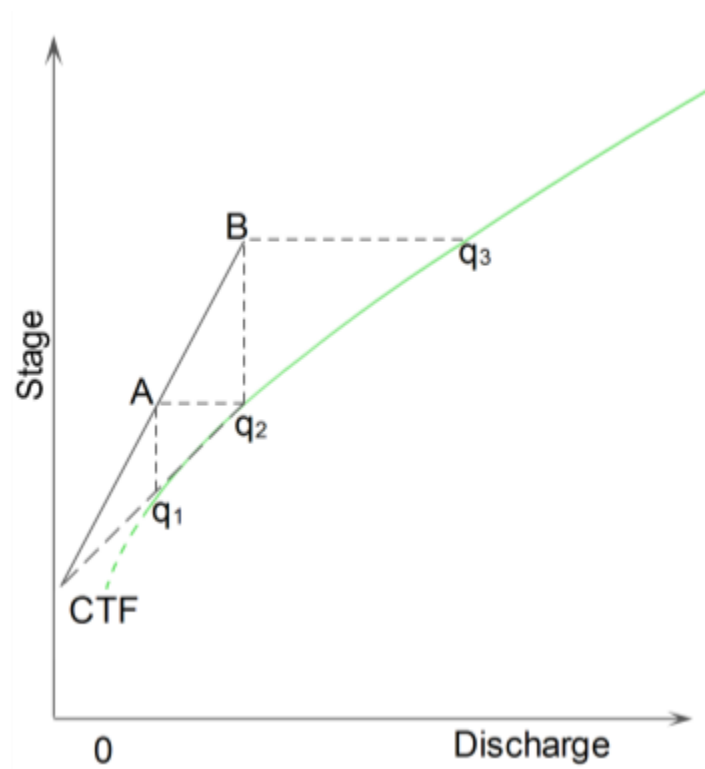
Figure 17 – Estimating cease to flow (CTF) from a partial rating curve plot
