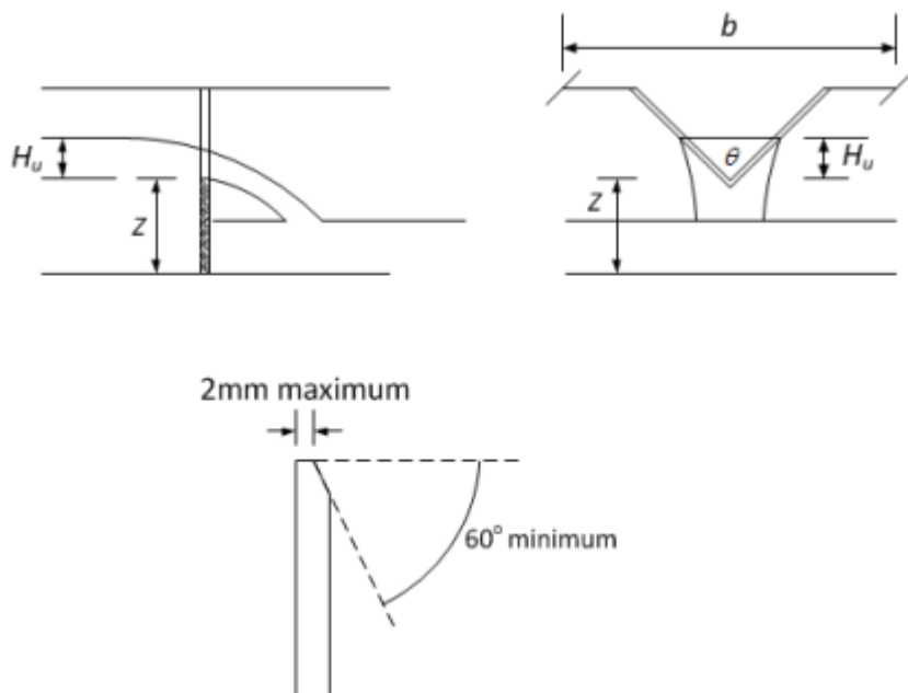
Figure 12 – V-notch Dimensions
