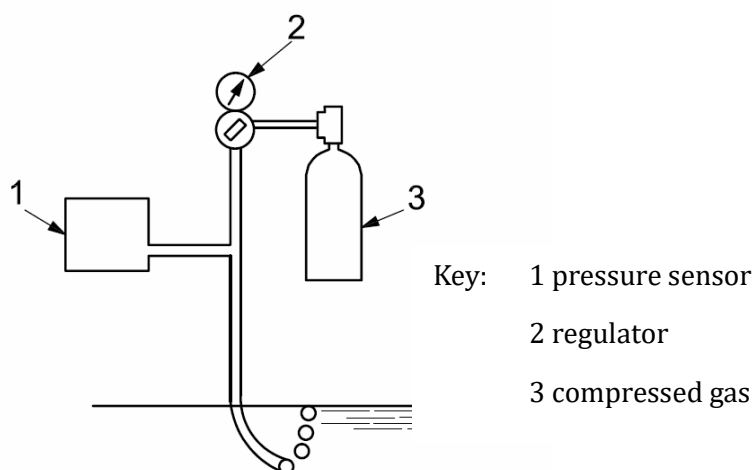
Figure 4 – Gas purge system.
