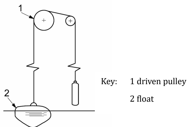
Figure 3 – Float and counterweight configuration.
