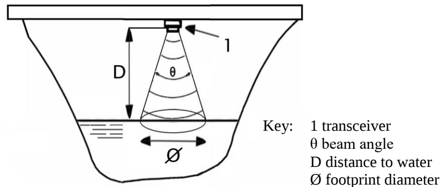
Figure 6 – Radar water level sensing configuration.
