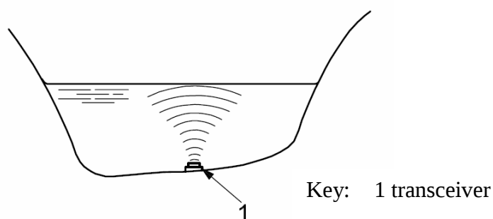
Figure 5 – Acoustic water level sensing – sound path in water.
