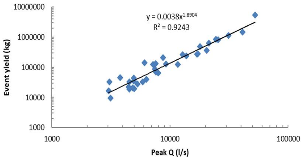
Figure 10-2 – Relation between event sediment load and event peak discharge for Waitomo River at Aranui Caves Bridge. Note even data scatter and linear trend on log-log plot, justifying use of a linear-regression model. The log-bias correction to be applied to the regression coefficient 0.0038, calculated by the Duan (1983) ‘smearing’ factor, is 1.08.
