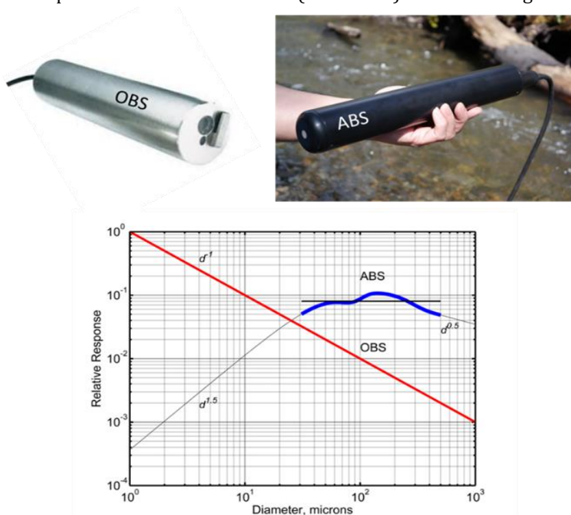
Figure 7-1 – Example ABS and OBS sensors, and their relative response to a given concentration of suspended sediment for different sediment sizes. The ABS is a LISST-ABS (Sequoia Scientific): it uses an acoustic frequency of 8 MHz, senses SSC at a point 5 cm from the transducer at the end of the instrument, and has a reasonably “flat” and strong response for sediment between 32 and 500 microns but is relatively insensitive to clay (finer than 4 microns). The OBS pictured is a HACH Solitax, which is ISO 7027: 2016-1–compliant and has a mechanical lens-wiper. The response of OBS sensors is inversely related to sediment size, so they are most sensitive to suspended clay but relatively insensitive to sand. Graph sourced from Sequoia Scientific, Inc.
