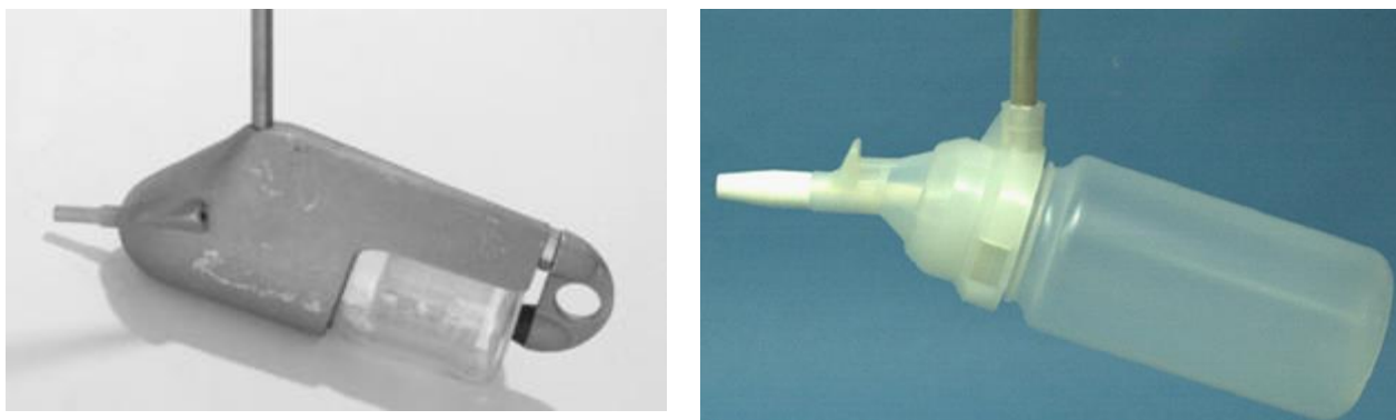
Figure 4-2 – Left: a DH-48 depth-integrating suspended sediment sampler mounted on a wading rod. Right: a DH-81 depth-integrating suspended sediment sampler mounted on a wading rod (photos: Gray and Landers, 2014).
