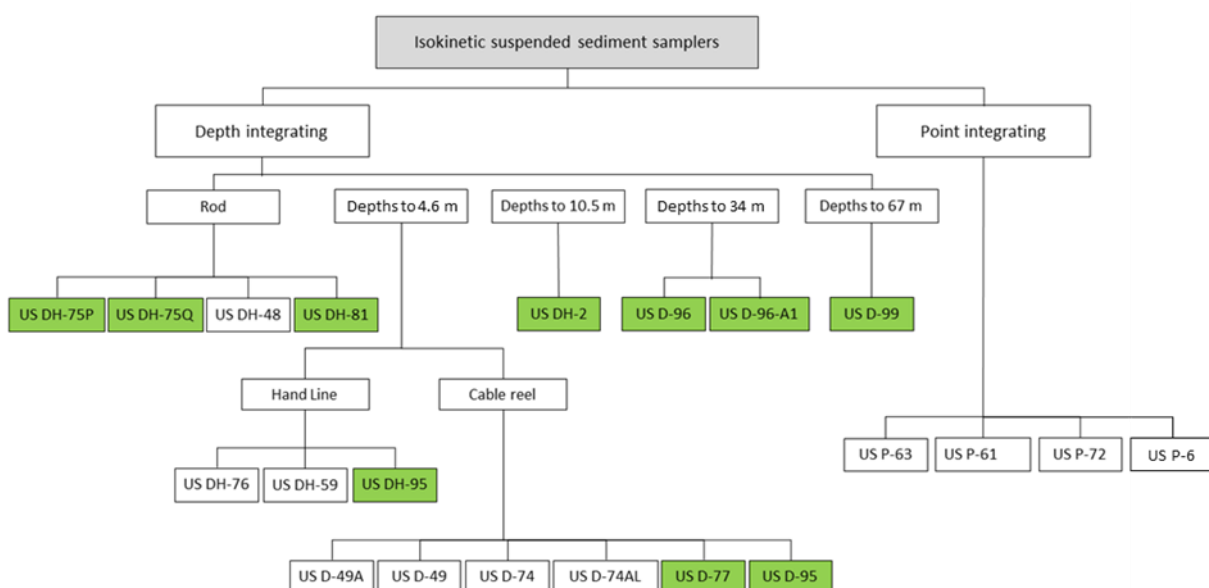
Figure 4-1 – Isokinetic suspended sediment samplers classified by type of deployment system and effective sampling depth. Green-filled boxes indicate samplers that can be used for trace-element water quality sampling as well as suspended sediment measurements.
