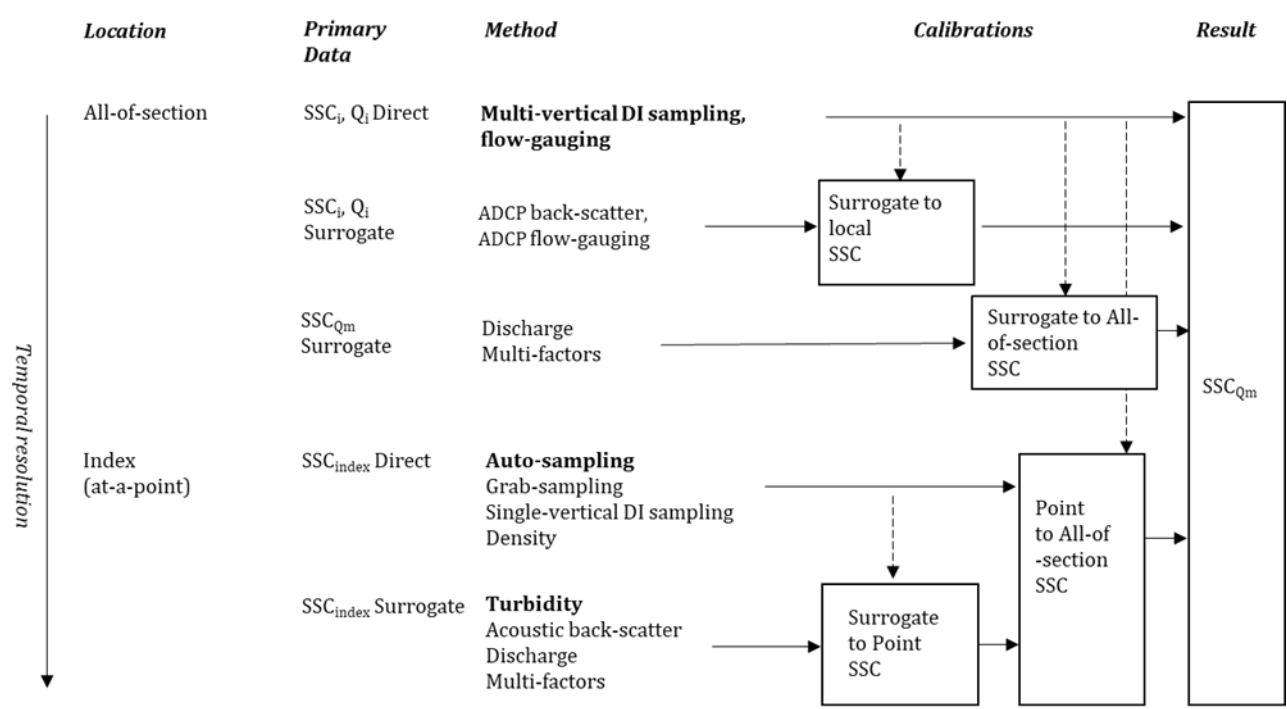
Figure 1-1 – Method pathways for determining flow-weighted, cross-section mean SSC ( SSC_{Qm} ) for the purpose of recording suspended sediment load. Bold font shows components of the method pathway based on use of a turbidity sensor as an SSC surrogate. i-suffixes indicate measurements made across multiple verticals or flow sections.
