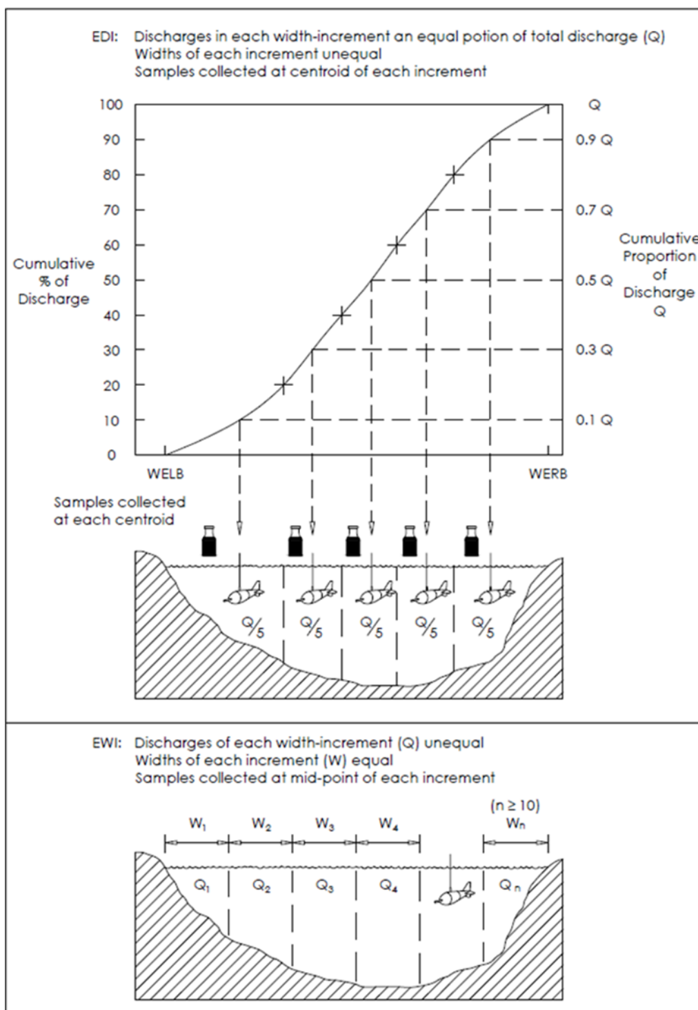
Figure 4-7 – Location of sampling verticals using the EDI and EWI methods. With EDI method (top), verticals are located at the centroids of sub-sections carrying equal portions of the total discharge. For EWI method (bottom), verticals are located at the midpoints of sub-sections that are equal in width.
