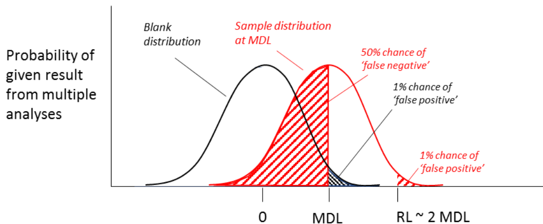
Figure 11-4 – Method Detection Limit (MDL) and Reporting Limit (RL) definitions. Analysis of blank samples provides a distribution of results (coloured black) centred about zero. The MDL is where there is only a 1% chance of a false positive value being detected. Analysis of a sample with actual value at the MDL (coloured red) has a 50% chance of the result being less than the MDL (i.e. a false negative). The RL is set so that there is only a 1% chance of a false exceedance of the MDL. This is approximated by RL = 2 \times MDL .
