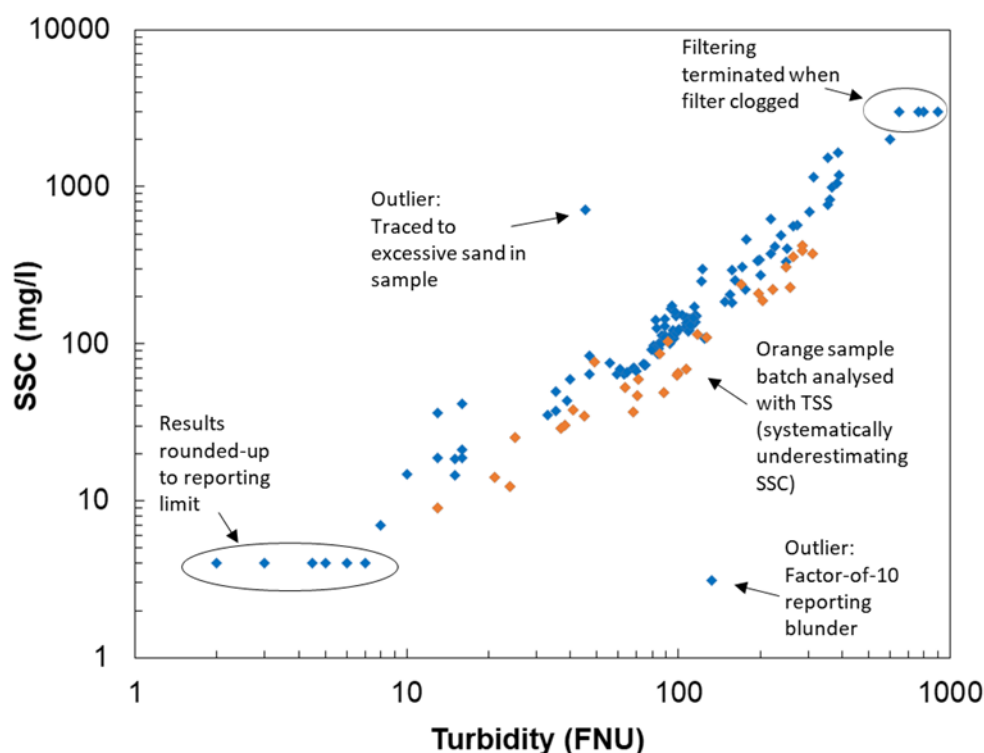
Figure 8-1 – A calibration plot relating SSC to turbidity, illustrating examples of suspect SSC data points. (i) High outlier point traced to unusually high sand mass in sample, suggesting sample corruption by bedform sampling, corroborated by site observations. (ii) Low outlier traced to a laboratory reporting
