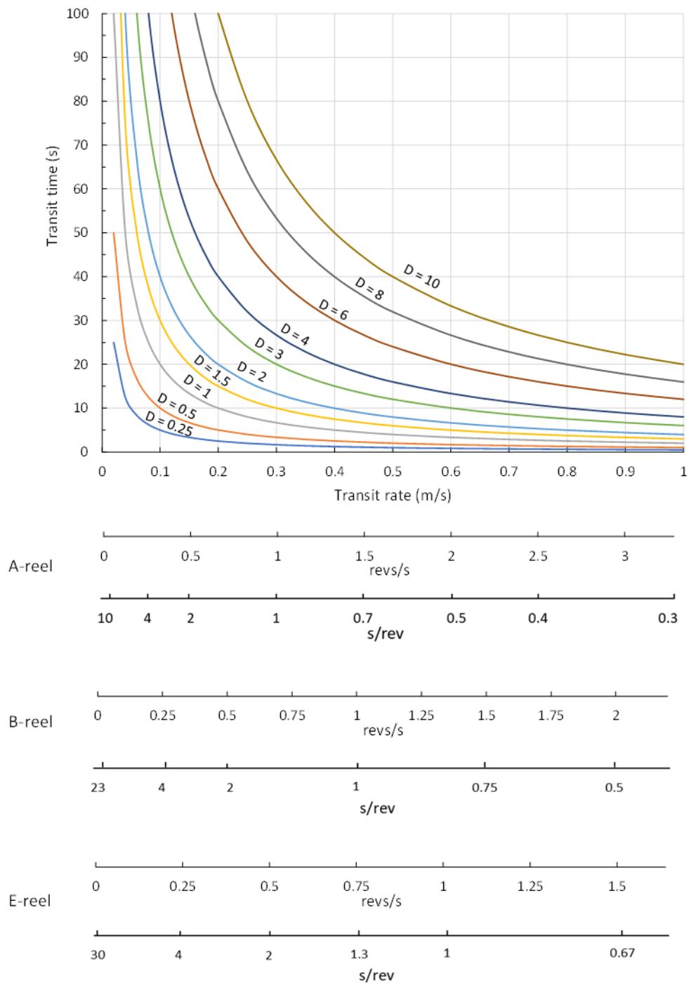
Figure 4-11 – Nomograph for converting transit time ( t ) to transit rate ( tR ) for a two-way traverse over different depths ( D ) using different sounding reels. Example: for t = 12 s and D = 2.0 m, tR = 0.34 m/s, which is equivalent to 1.1 revolutions per second or 0.9 seconds per revolution for an A-reel.
