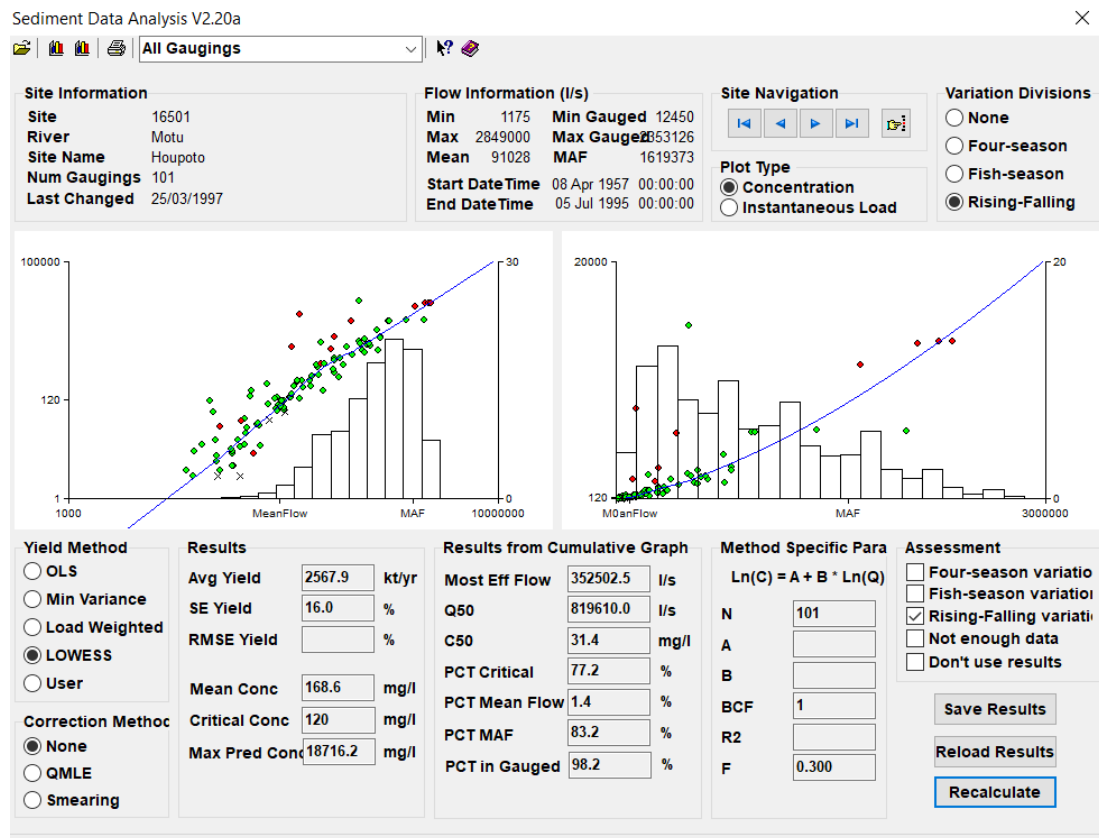
Figure F-1 – Example of steps and checks when fitting a sediment rating curve, illustrated for the Motu River at Houpoto dataset with the desktop displayed by the rating-fitting software SEDRATE. Data plots on log (left graph) and linear (right graph) scales show more uniform data scatter with log transformation. On log scales, the trend is reasonably linear so either a least-squares or LOWESS fit could be chosen (LOWESS is selected in this case). The maximum predicted SSC is 18,712 mg/l, which is reasonable for the Motu catchment. Sample density aligns reasonably with the load distribution (bar graphs). 98.2% of the estimated load (2,567,900 t/yr) is transported at discharges within the sampled range. Thus, the discharge-targeting sampling strategy is reasonable. Rising stage points tend to plot higher than falling stage points, thus it is important to keep the rising stage point count in proportion to the duration of rising stages. Alternatively, if there is a strong separation of rising and falling stage points, separate rising-stage and falling-stage rating curves could be fitted.
