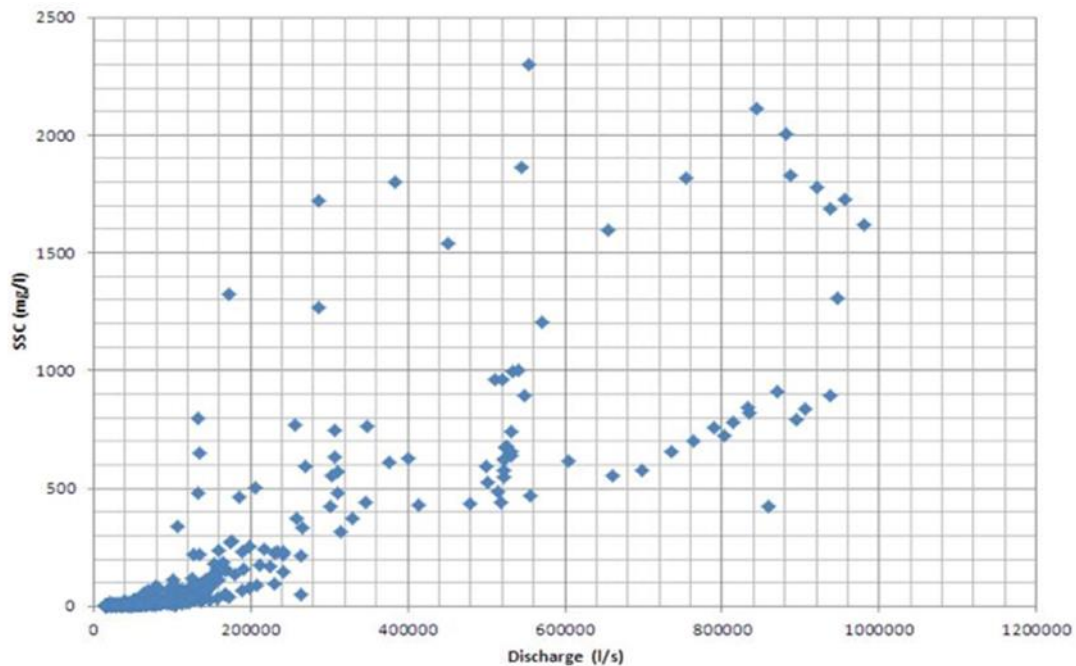
Figure D-2 – Example plot of discharge versus suspended sediment concentration (SSC). Note wide scatter associated with loop ratings during discrete events.
