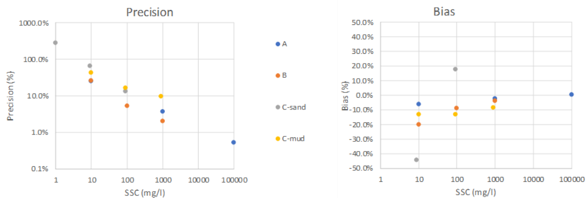
Figure 11-2 – Precision and bias of ASTM Methods A, B, and C as reported by ASTM (2019).
