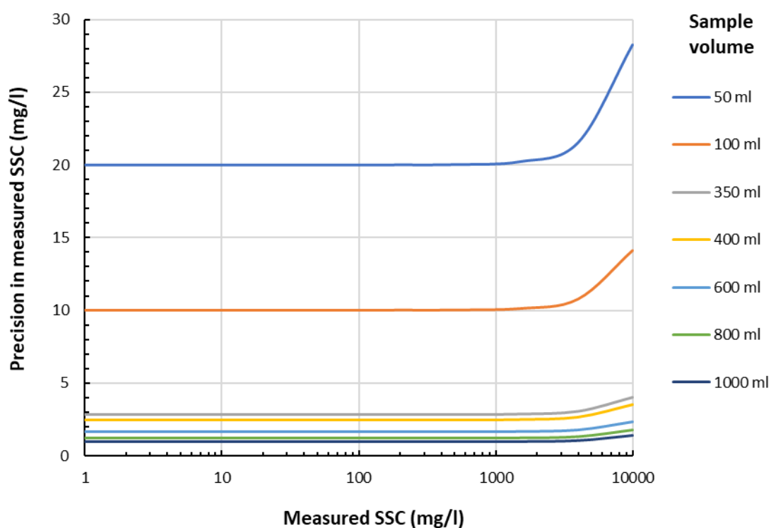
Figure 11-3 – Theoretical precision (i.e. range of results from repeat measurements) in total SSC associated with ASTM filter analysis of sand and mud splits in relation to sample volume and SSC. Note how precision quality degrades as sample volume decreases and as SSC increases above about 3500 mg/l.
