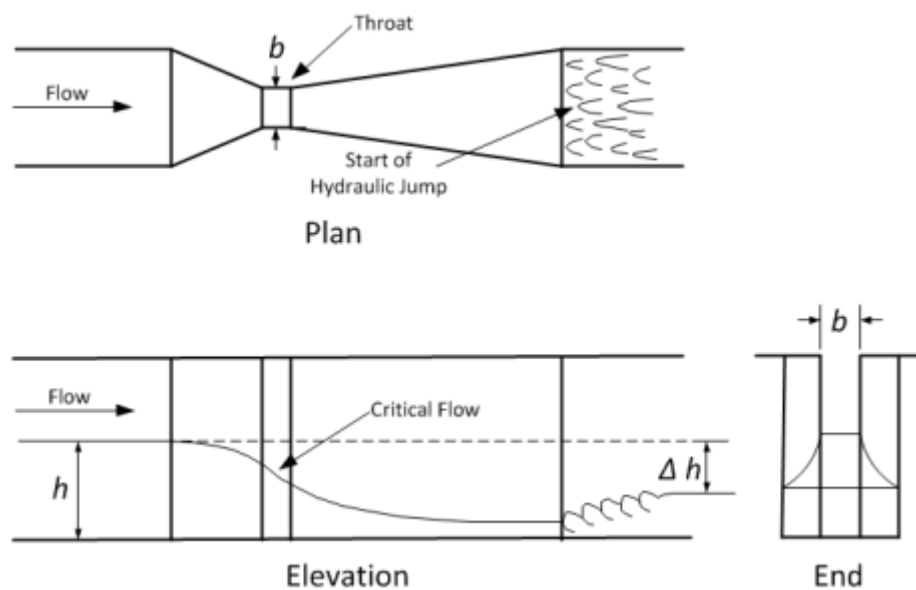
Figure 14 – Typical Flume
