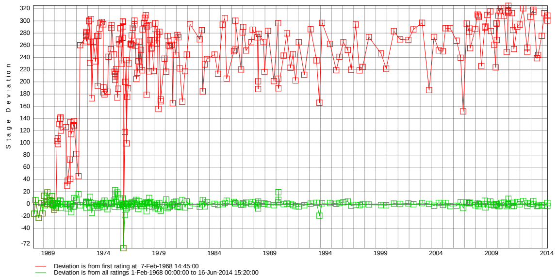
Figure 39 – ‘Before and after’ bed plot
