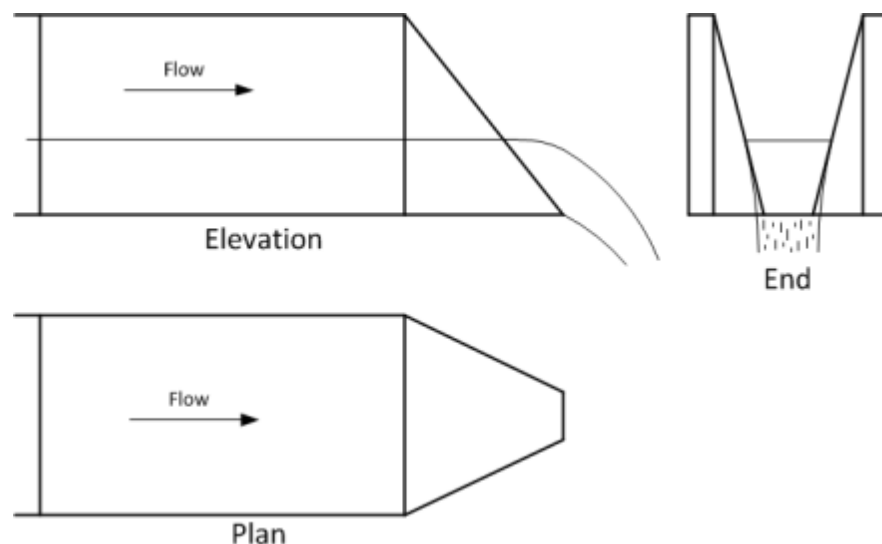
Figure 17 – H-Flume configuration
