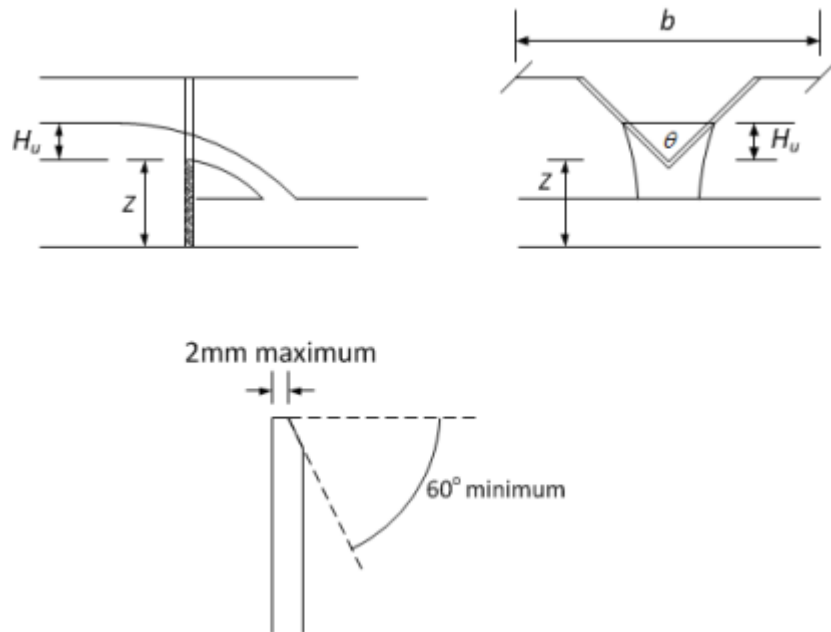
Figure 13 – V-notch Dimensions
