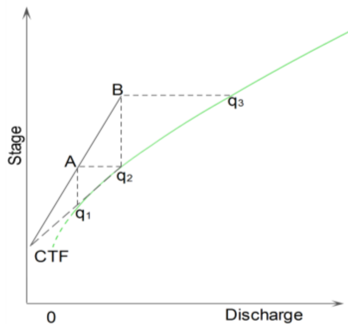
Figure 18 – Estimating cease to flow (CTF) from a partial rating curve plot
