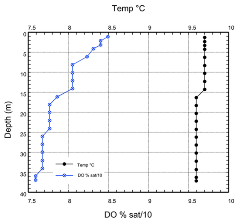
Figure 2 – An example of a water temperature-DO depth profile for a lake in isothermal condition
