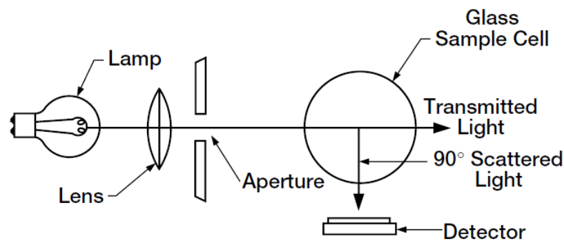
Figure 4 – Schematic of the key components of a turbidity sensor
