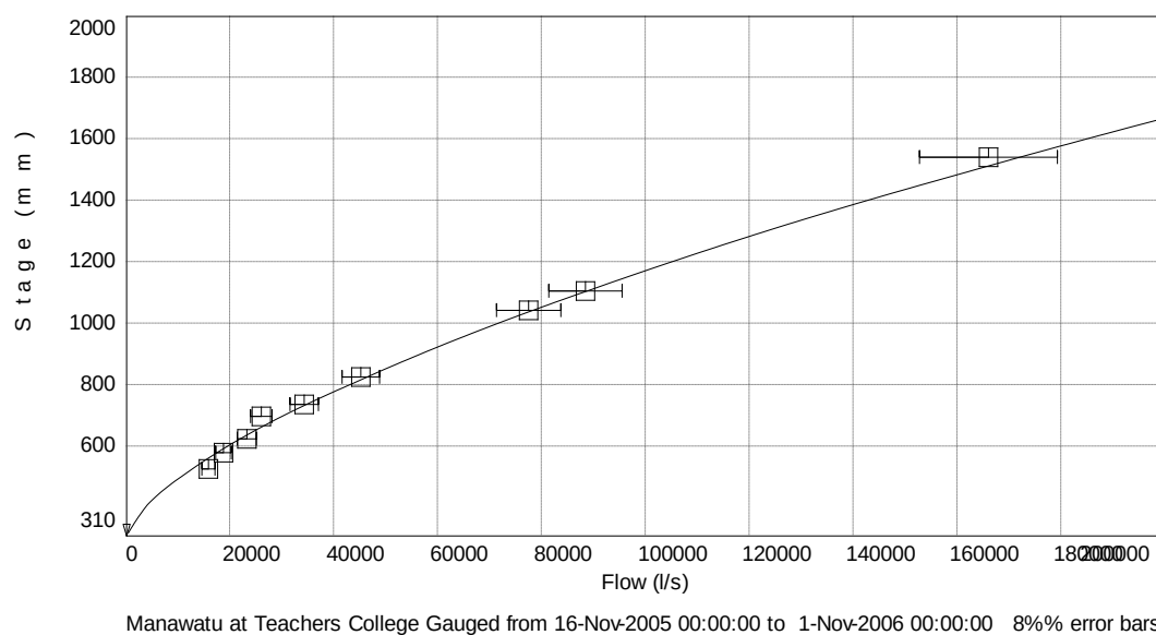
Figure 33b – Final theoretical bottom-end rating curve for Manawatu at Teachers College, shown with actual discharge measurements within the period of stable control during which the cross-sections used to derive the rating curve were surveyed
