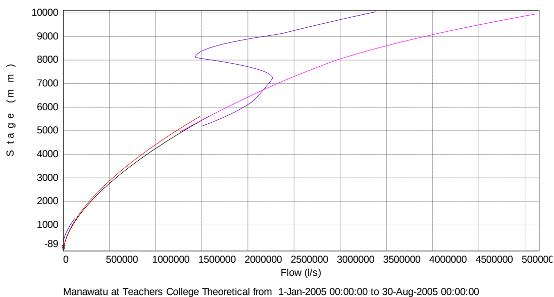
Figure 31 – Theoretical rating segments for Manawatu at Teachers College for low, mid-range and high flows
