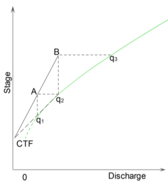
Figure 18 – Estimating cease to flow (CTF) from a partial rating curve plot
