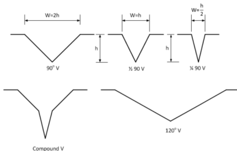
Figure 12 – V-Notch Weir Cross-Section Profiles
