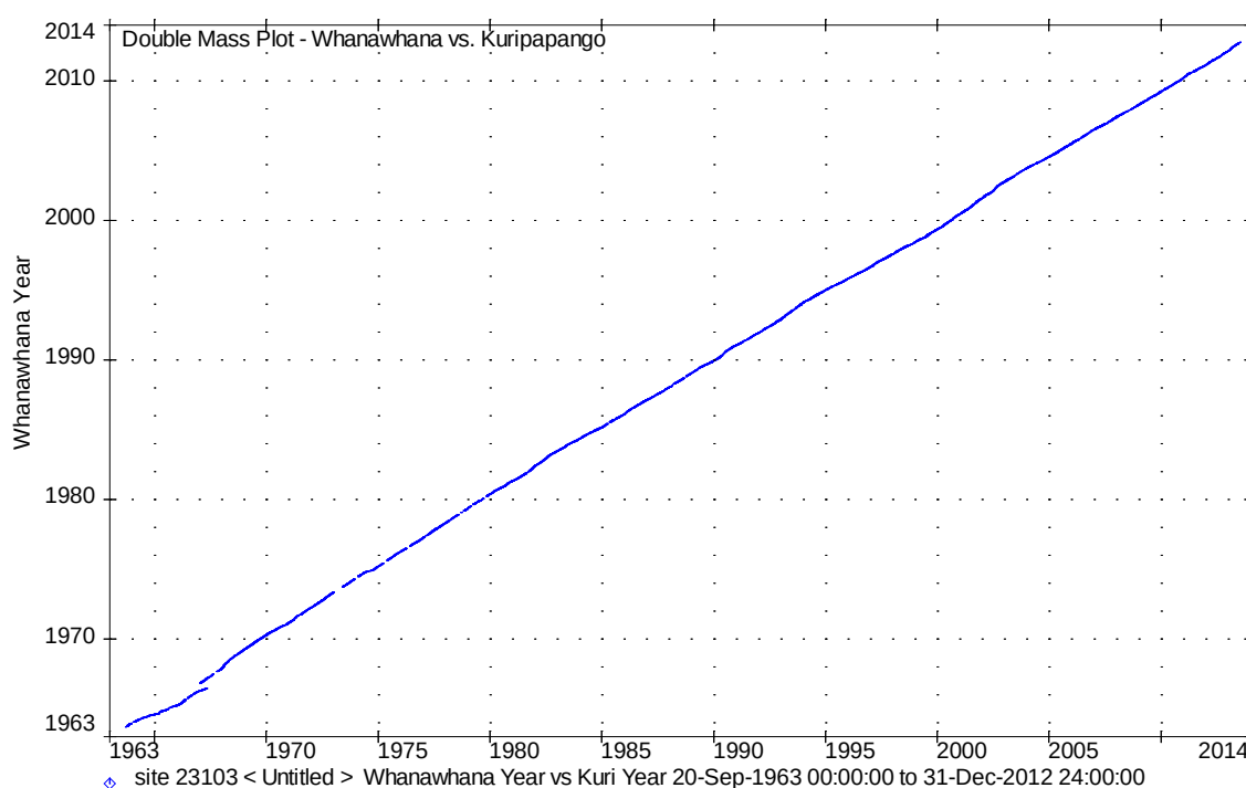
Figure 40 – Double mass flow plot
