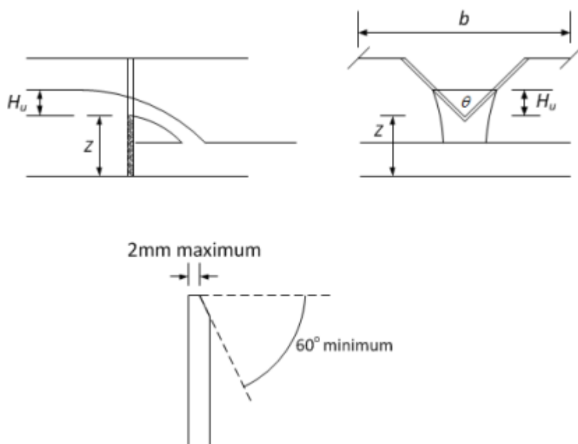
Figure 13 – V-notch Dimensions
